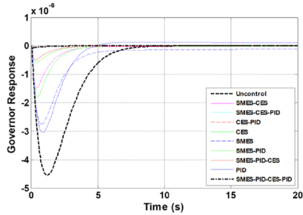
Figure 12. Governor response under different scenarios.
