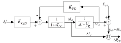
Figure 6. Blok Diagram CES
