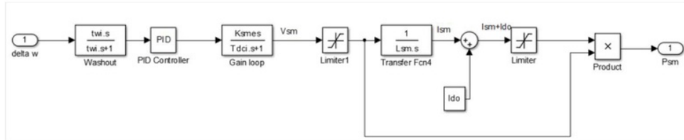
Figure 8. Simulink model of SMES.
