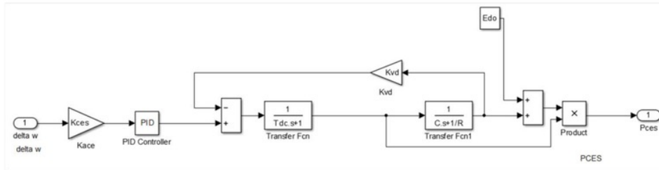
Figure 9. Simulink model of CES
