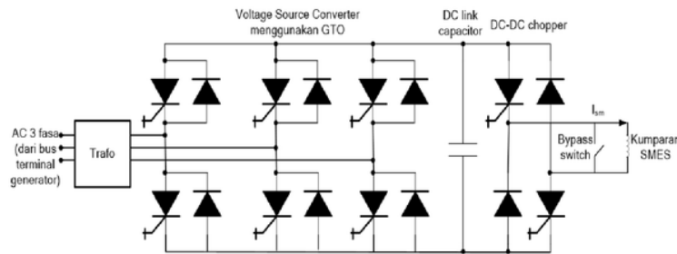
Figure 3. SMES configuration.
