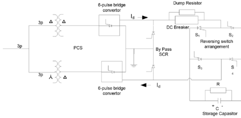
Figure 5. Schematic diagram of capacitor Energy Storage.
