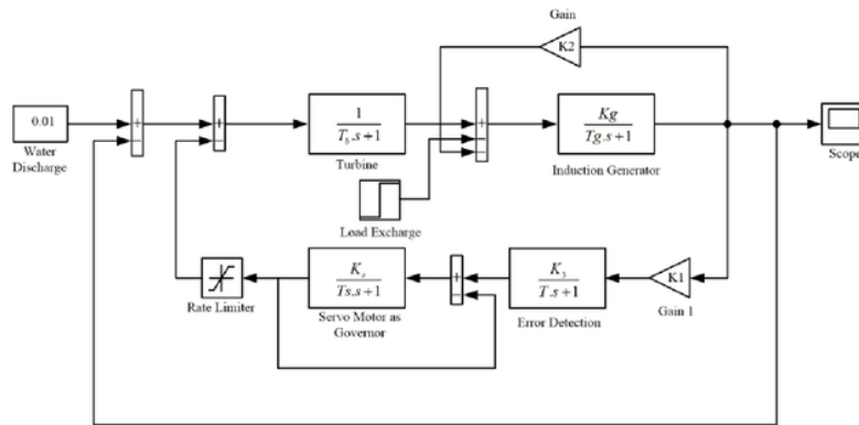
Figure. 1. Block diagram of micro hydro.
