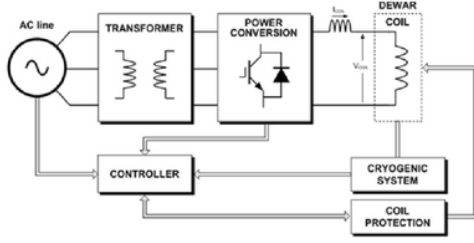
Figure 2. Schematic diagram of SMES
