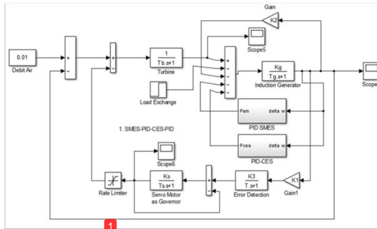
Figure 7. Simulink model of entire system.
